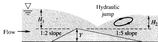
Fig. P10.122 The Crump weir [19, chap. 4]
