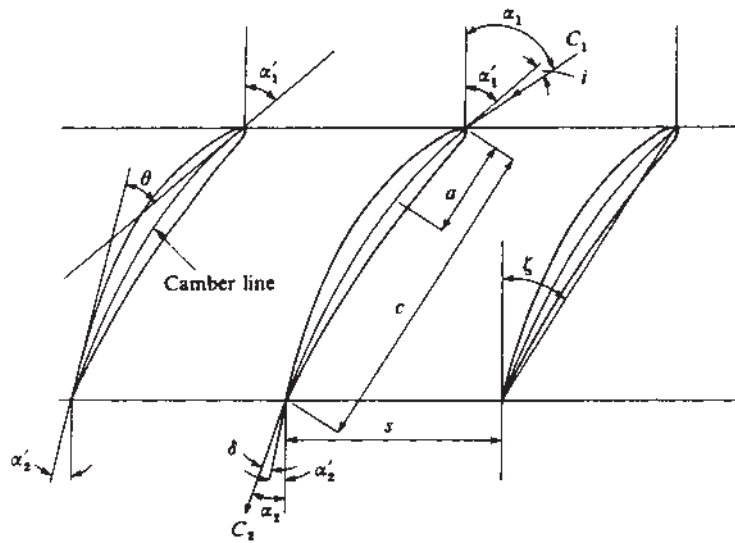
Figure 5.7 Cascade nomenclature.
